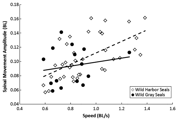
Figure 9. Plot indicating the relationship between spinal amplitude and speed (BL/s) of the wild harbor ( y = 0.08x + 0.03 , r = 0.6 , P < 0.001 ; dashed line) and gray seals ( y = 0.03x + 0.07 , r = 0.2 , ns; solid line).
