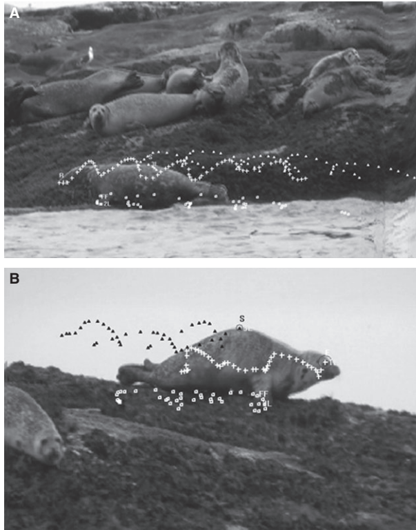
Figure 7. Feature tracking of a harbor seal (bottom) and gray seal (top) across a beach on Duck Island. Specific points were tracked over multiple strides, including the maximum point of the dorsal margin of the body during progression (solid triangles), the rostrum (crosses), and the tip of the fore flippers (open squares).
