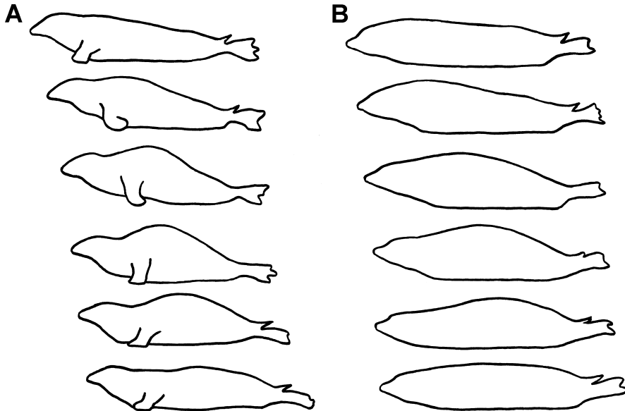
Figure 2. Lateral view of movements over one stride cycle for captive gray seal (A, Kjya) and harbor seal (B, Spanky) moving over a level concrete surface. The sequences are tracings from video recordings at intervals of 0.067 s. The sequence is initiated from the bottom of the figure.
