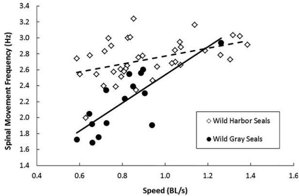
Figure 8. Plot indicating the relationship between spinal frequency (Hz) and speed (BL/s) of the wild harbor ( y = 0.50x + 2.28 , r = 0.45 , P = 0.006 ; dashed line) and gray seals ( y = 1.76x + 0.78 , r = 0.79 , P < 0.001 ; solid line).
