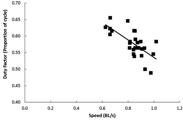
Figure 6. Scatterplot representing duty factor against speed (BL/s) for the captive gray seals ( y = -0.26x + 0.80 , r = -0.69 ).
