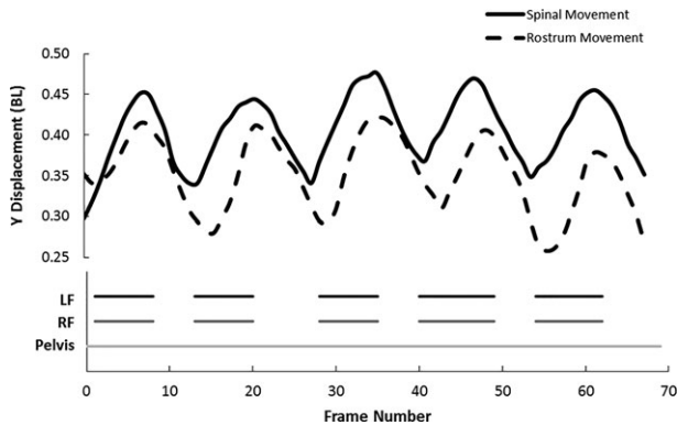
Figure 11. Sinusoidal patterns of the rostral tip and spine that were created by the undulatory movement along with the footfall pattern of the fore flippers (right fore flipper = RF; left fore flipper = LF) and pelvis with the frame number. With the exception of the one captive harbor seal, all seals included in this study displayed relatively similar patterns and footfall sequences.
