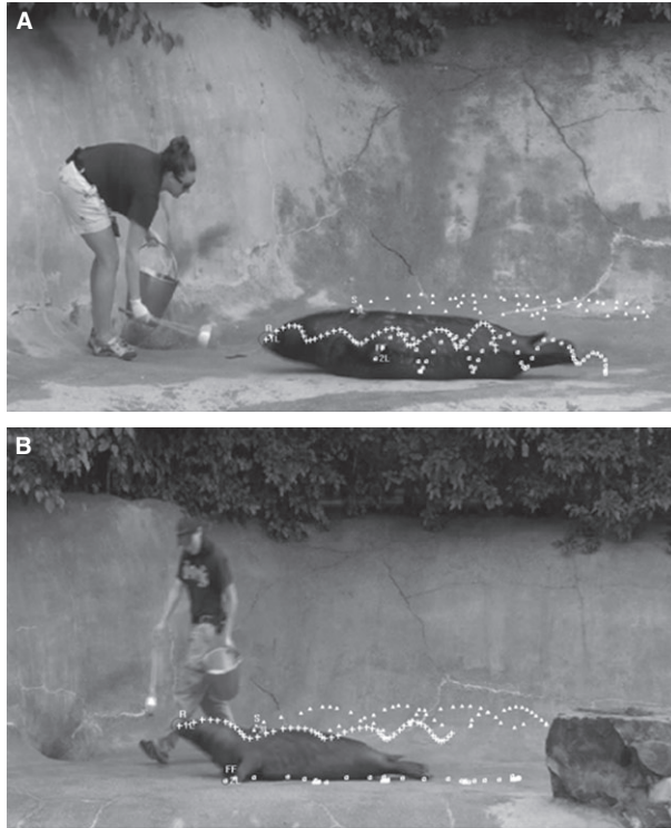
Figure 3. Feature tracking patterns of the captive harbor seal (top, Spanky) and gray seal (bottom, Kja) moving over a level concrete surface. Specific points were tracked over multiple strides, including the maximum point of the dorsal margin of the body during progression (solid triangles), the rostrum (crosses), and the tip of the fore flippers (open squares).
