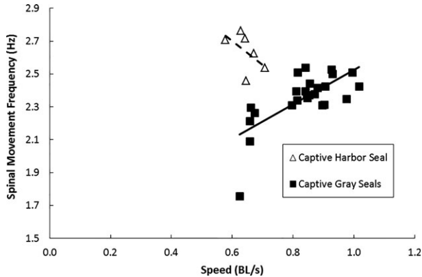
Figure 4. Scatterplot displaying the frequency (Hz) of the dorsal margin of the body against speed (BL/s) for captive harbor ( y = -1.46x + 3.57 , r = -0.54 ; dashed line) and gray seals ( y = 1.05x + 1.48 , r = 0.70 ; solid line).
