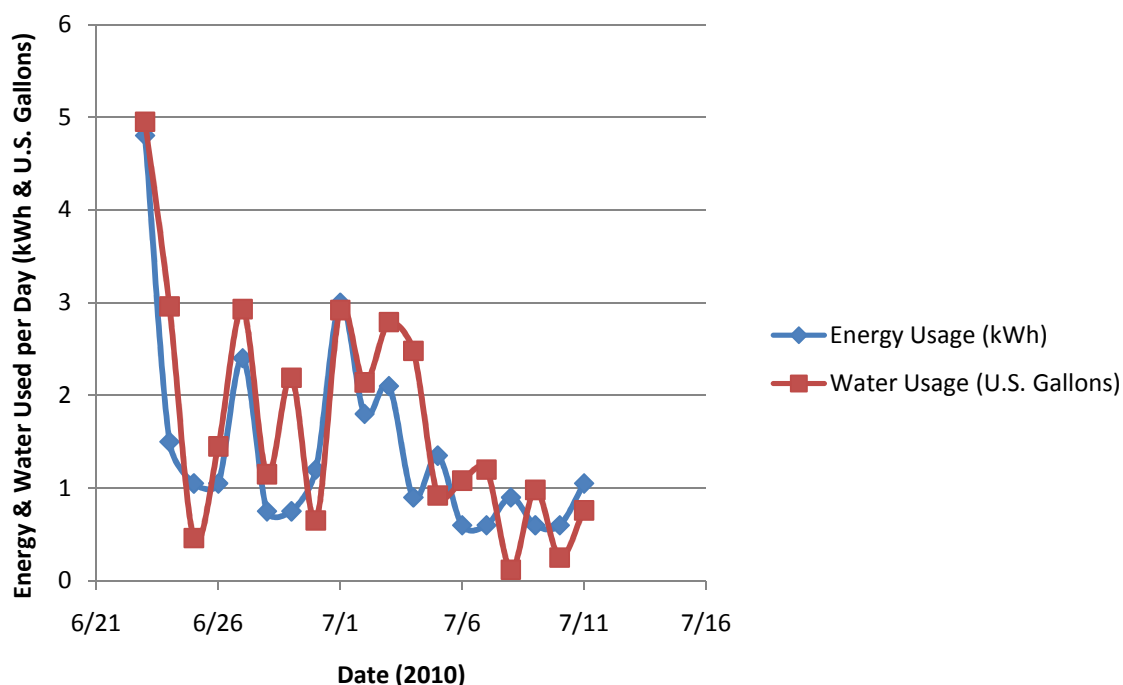
Figure 17: Energy and Water Usage of Palmer-Kinne Electric Water Heater per Day
