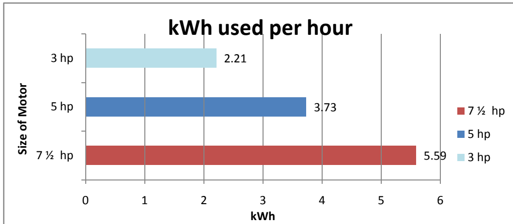
Figure 23: Energy Consumption Comparison (7 ½ hp, 5 hp, 3 hp)
